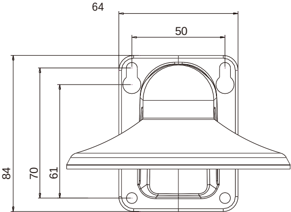
Measurements(Unit:mm)
